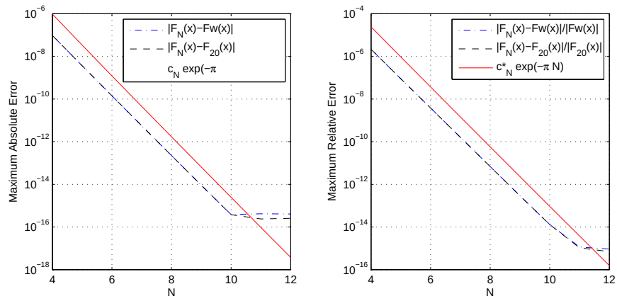
Fig. 1 Left hand side: maximum error, \max_{x \in [0, 2\pi]} |F(x) - F_N(x)| , and its upper bound (12) (13), plotted against N , where F(x) is approximated by Fw(x) := e^{ix^2} w_{36}(e^{i\pi/4} x) = 2 with w_{36}(x) = \sum_{k=0}^{35} \frac{(-1)^k}{k!} x^k .
