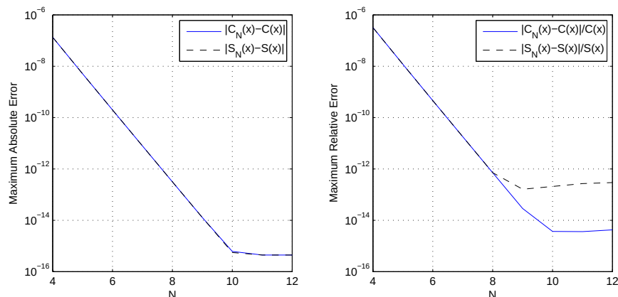
Fig. 4 Left hand side: maximum values of |jC_N(x) - C(x)| and |jS_N(x) - S(x)| on 0 \leq x \leq 20 . Right hand side: maximum values of |jC_N(x) - C(x)|/|C(x)| and |jS_N(x) - S(x)|/|S(x)| on 0 \leq x \leq 20 .
