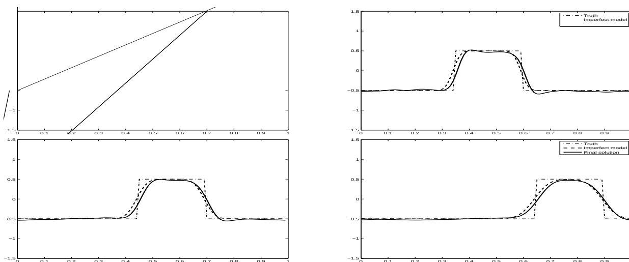
Figure 14. Results for 4DVar for a shifted (and noisy) background and for background error covariance matrix B taken from (29) with \sigma_b^2 = 0.01
