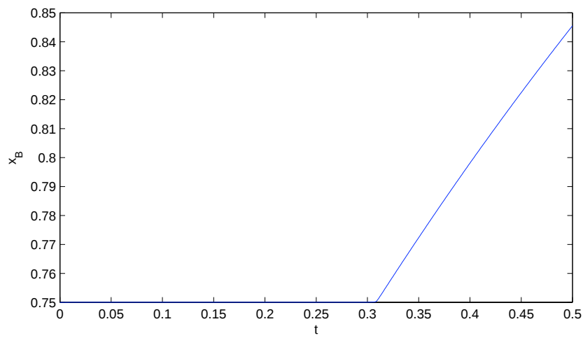
Figure 8.4: Movement of the boundary of the PME with n = 1 , \epsilon = 4:5
