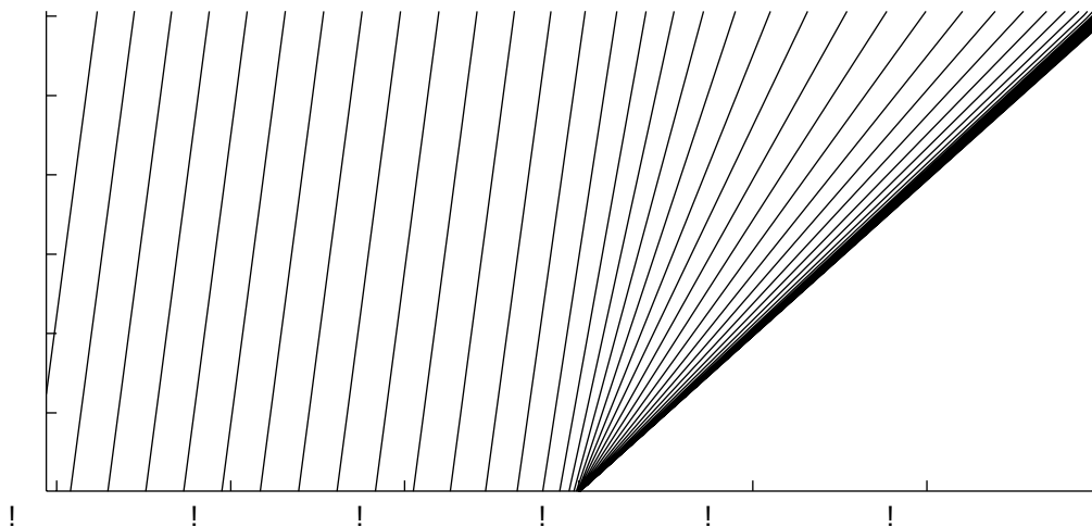
Figure 8.6: Close up of the moving boundary of the numerical solution to the PME with n = 7 , \alpha = 0.5
